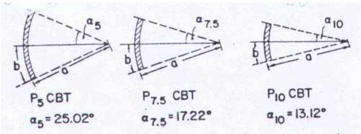
Fig. 2. Geometry of P_5 CBT (left), P_{7.5} CBT (center), and P_{10} CBT (right) spherical cap constant-beamwidth transducers. (Reproduced from Fig. 1 of [7].)
